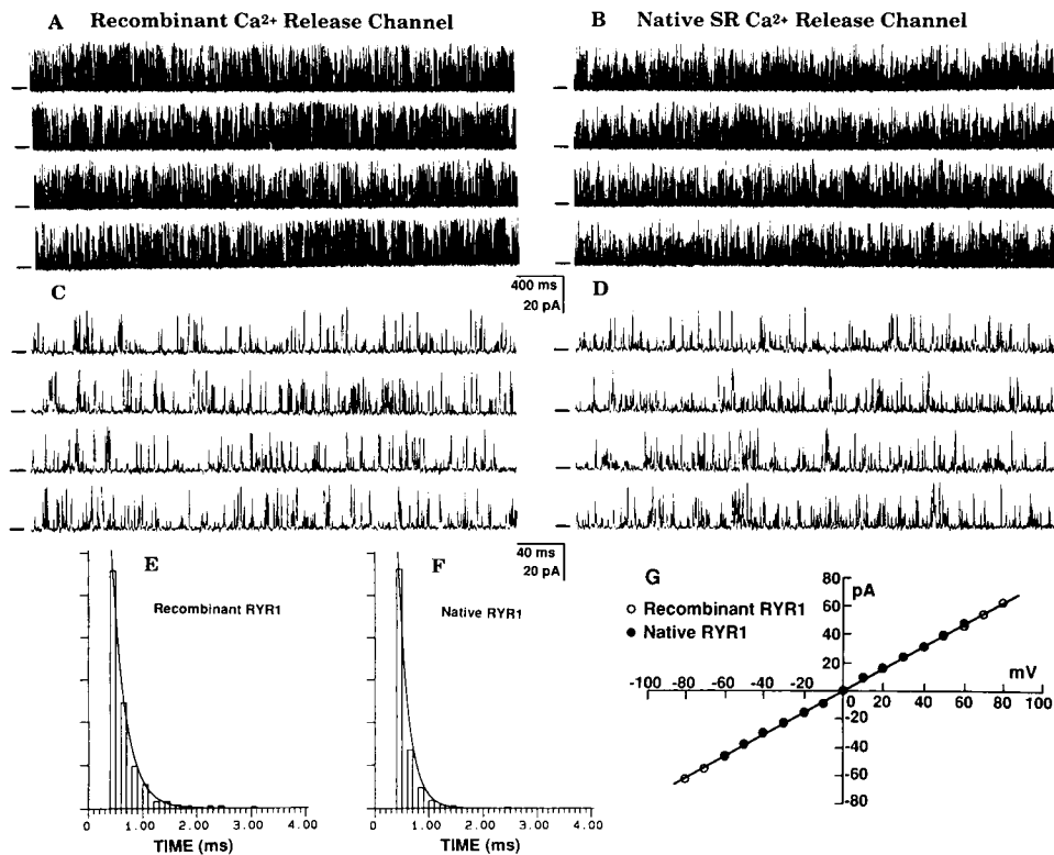
FIGURE 2 Comparison of single-channel properties of recombinant and native single \text{Ca}^{2+} release channels. Sucrose density gradient-purified ryanodine receptors from rabbit skeletal muscle heavy sarcoplasmic reticulum vesicles and microsomal membranes of HEK-293 cells transfected with skeletal muscle ryanodine receptor cDNA were incorporated into lipid bilayers as described in Materials and Methods. The trans chamber was connected to the headstage input of an amplifier. The cis chamber was held at virtual ground. In this experiment, the luminal ( trans ) potentials were varied and reported. A symmetrical recording solution containing 250 mM KCl and 25 mM HEPES (pH 7.4) was used for all recordings. Recordings were filtered at 1 kHz and digitized at 5 kHz. Both native and recombinant single \text{Ca}^{2+} channels were first inhibited by 0.1 mM EGTA ( cis ) and then reactivated by 0.1 mM \text{CaCl}_2 ( cis ), indicating that the cytoplasmic face of the channel was located in the cis chamber. Single-channel current fluctuations of the recombinant and native channels in the presence of 2.5 \mu\text{M} free \text{Ca}^{2+} (0.1 mM EGTA plus 0.1 mM \text{CaCl}_2 ) at +30 mV are shown in A and B, respectively. Current traces illustrated in C and D are taken from A and B and shown in a 10-fold shorter time scale. Baselines are indicated by lines to the left of each current trace. Continuous recordings are shown in each panel. Dwell-time histograms of open events of recombinant and native channels are illustrated in E and F, respectively. The average open time constant is 0.224 \pm 0.027 ms (mean \pm SD) ( n = 4 ) for the recombinant channel and 0.220 \pm 0.022 ms (mean \pm SD) ( n = 4 ) for the native channel. The y-axes in the dwell-time histograms E and F correspond to 52 events/division. (G) Current-voltage ( I-V ) relationship of the recombinant channel ( \circ ) and native channels ( \bullet ). Both display a linear relationship with slope conductances of 780 \pm 12.8 pS (mean \pm SD) ( n = 3 ) for the recombinant channel and 778 \pm 5.66 (mean \pm SD) ( n = 2 ) for the native channel.
