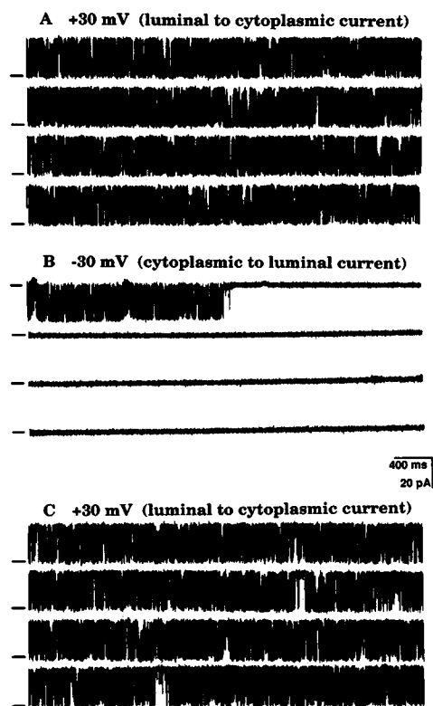
FIGURE 6 Asymmetrical blockade of recombinant single \text{Ca}^{2+} release channels. A spontaneous channel activity was inactivated by cis 0.21 mM EGTA, reactivated by cis 0.21 mM \text{CaCl}_2 , and further activated by cis 2.0 mM ATP, indicating that the cytoplasmic face of the channel lies in the cis chamber. In this experiment, the luminal ( trans ) potentials were varied and reported. (A) Single-channel currents recorded at +30 mV in symmetrical 250 mM KCl. Openings are upward and baselines are indicated by lines on the left of each current trace. Under these conditions, the direction of the current flow was from the luminal to the cytoplasmic side of the channel. Long-lived closed events were rare under these conditions. (B) Single-channel currents shortly after the voltage was changed from +30 mV to -30 mV. Openings are downward and baselines are marked. At -30 mV, current flowed from the cytoplasmic to the luminal side. Note that the channel was completely closed after opening for several seconds at -30 mV. Single-channel currents recorded after the voltage was changed from -30 mV back to +30 mV are shown in C. Openings are shown as upward deflections. Note that the channel was reactivated at +30 mV. A 16-s continuous recording is shown in each panel; all recordings are from the same channel.
